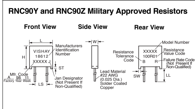
FIGURE 3 - IMPRINTING AND DIMENSIONS
